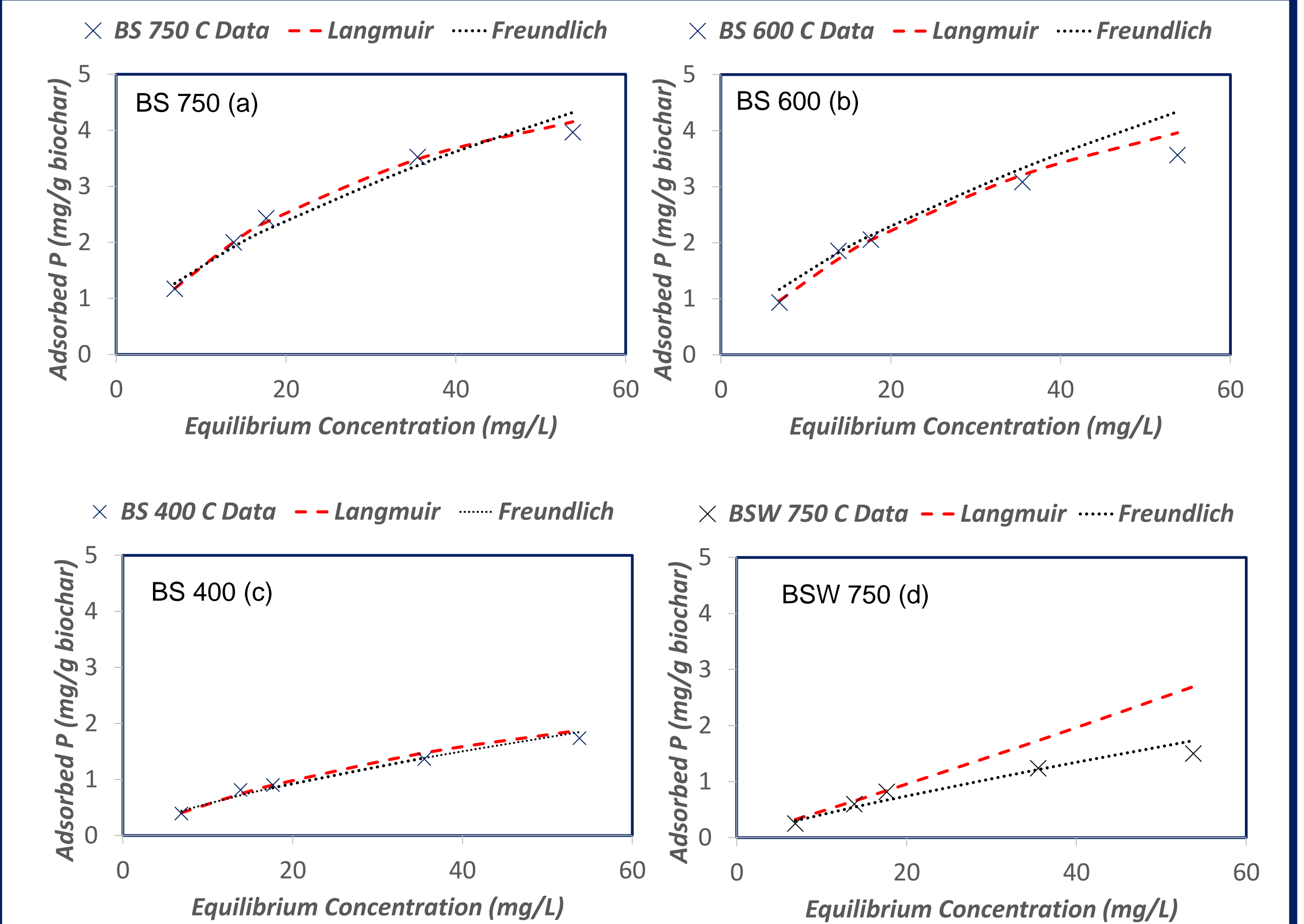
Fig 4. P adsorption isotherms and models by biosolid-derived biochars produced at 400, 600 and 750°C. (a) BS750, (b) BS600 (c) BS400, and (d) BSW750 (Washed). The red dash line represents the Langmuir isotherm model and the black dotted line represents the Freundlich isotherm model
