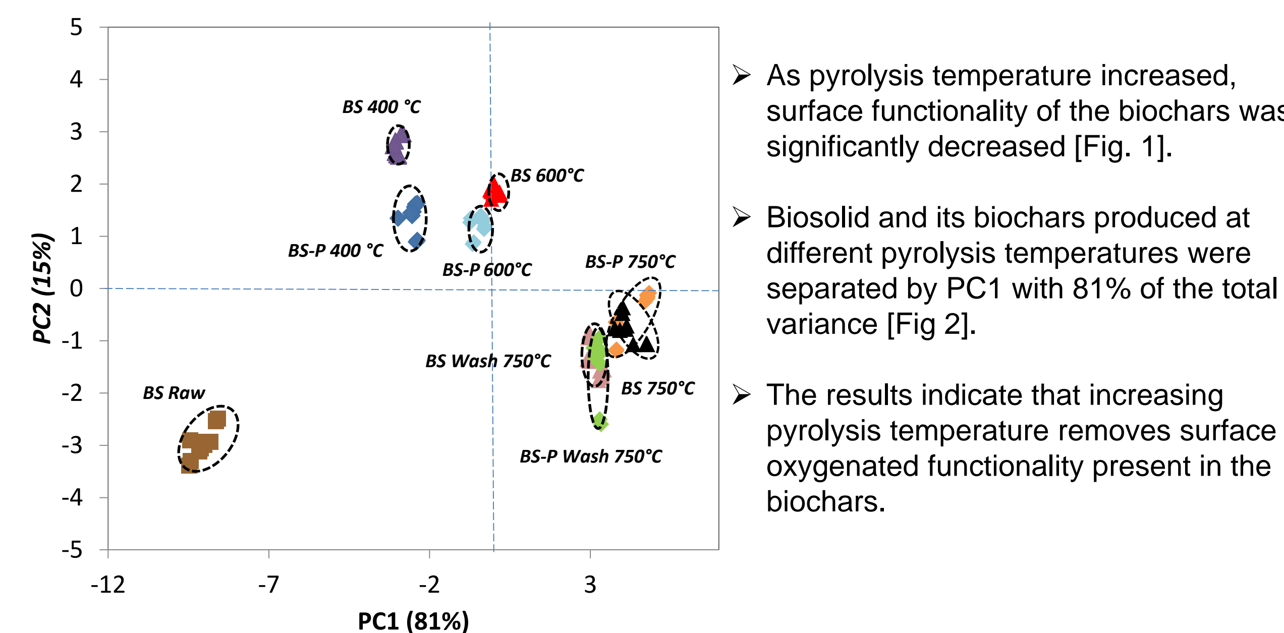
Fig. 2. PCA of FTIR spectra data
