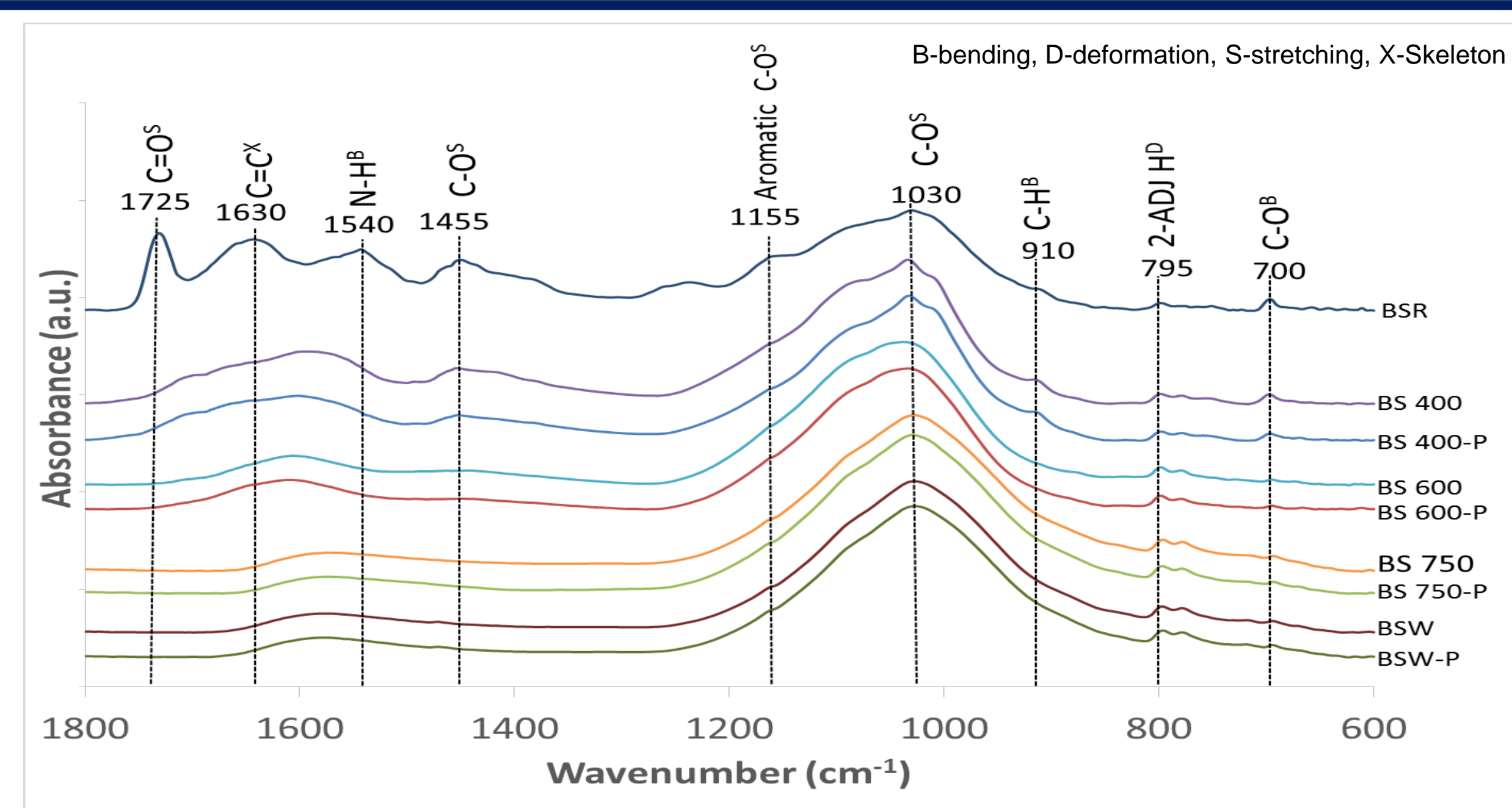
Fig. 1. FTIR spectra of the feedstock
