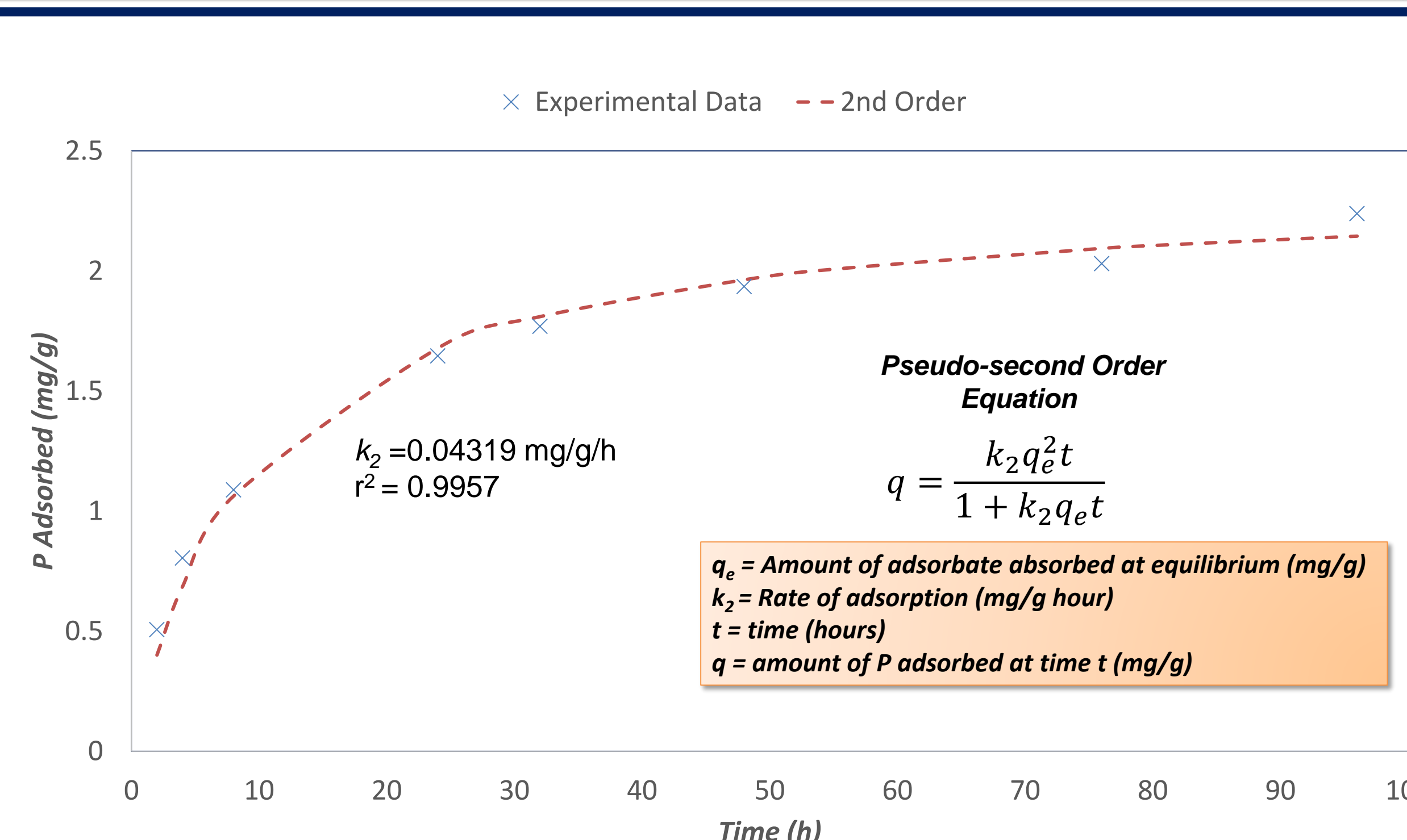
Fig. 3. Adsorption kinetics of P on BS750 and the fitted model using the pseudo-second order model
