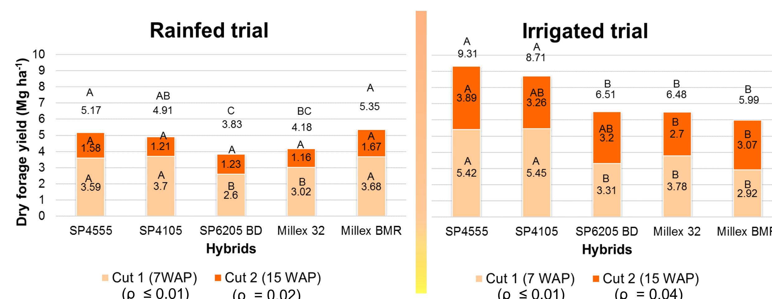
Figure 4: Dry forage yield among hybrids. Letters denote significant differences within same cut or total yields.
