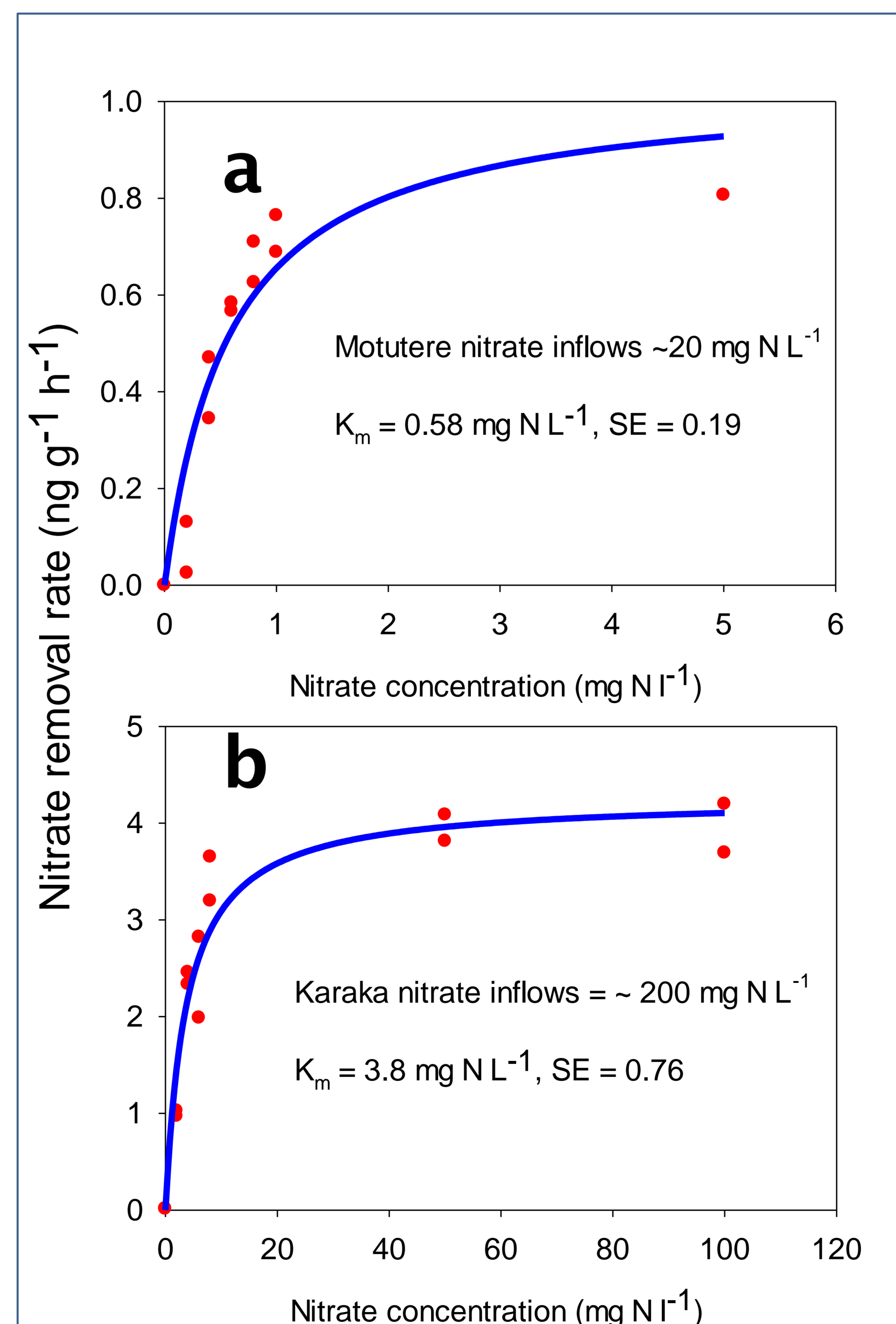
Fig 2. Dependence of nitrate removal on nitrate concentration from two denitrification beds (a) Motutere and (b) Karaka. K_m values are given on each plot. Note difference in nitrate concentrations between beds.
