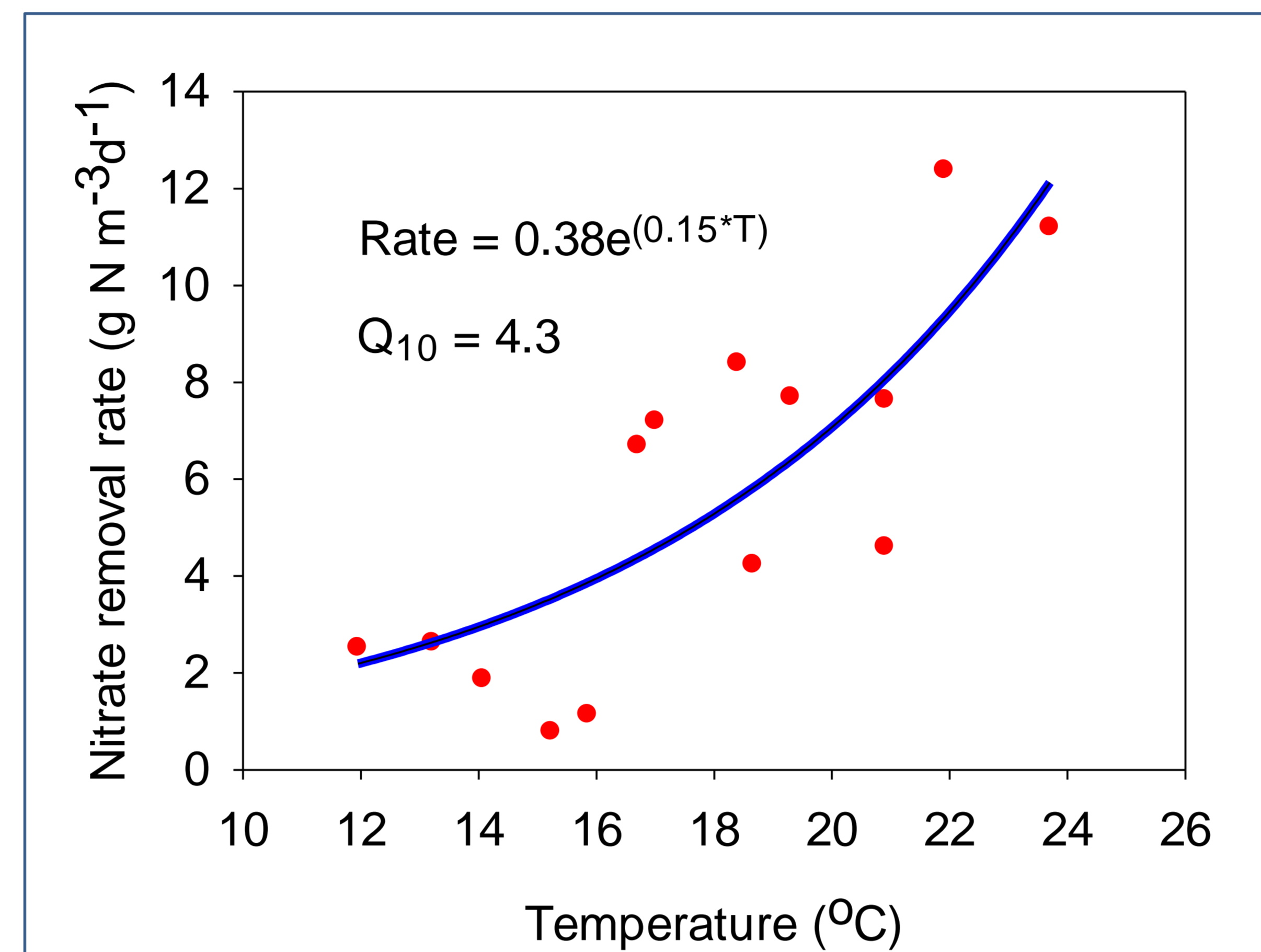
Fig. 1. Nitrate removal as a function of temperature at Karaka.
