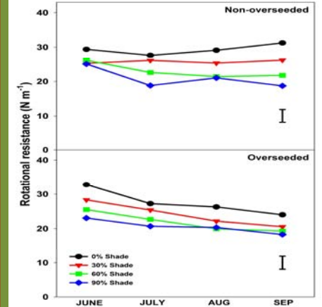
FIGURE 2. Rotational resistance over the 2014 growing season as affected by various shade levels. Error bar represents least significant difference between means (P=0.05).
