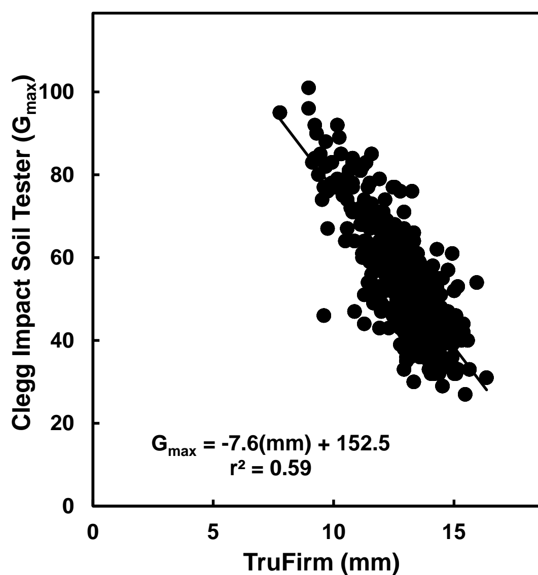
Fig. 1: All corresponding firmness measurements from 2017 using Clegg Impact Soil Tester (CIST) and FieldScout TruFirm meter. A highly significant linear relationship ( P < 0.0001 ) was observed from a total of 2508 paired measurements; CIST ranged from 27 to 101 G max ( \bar{x} = 53 ); TruFirm ranged from 8 to 16 mm ( \bar{x} = 13 ). A single drop per location was made with each device.
