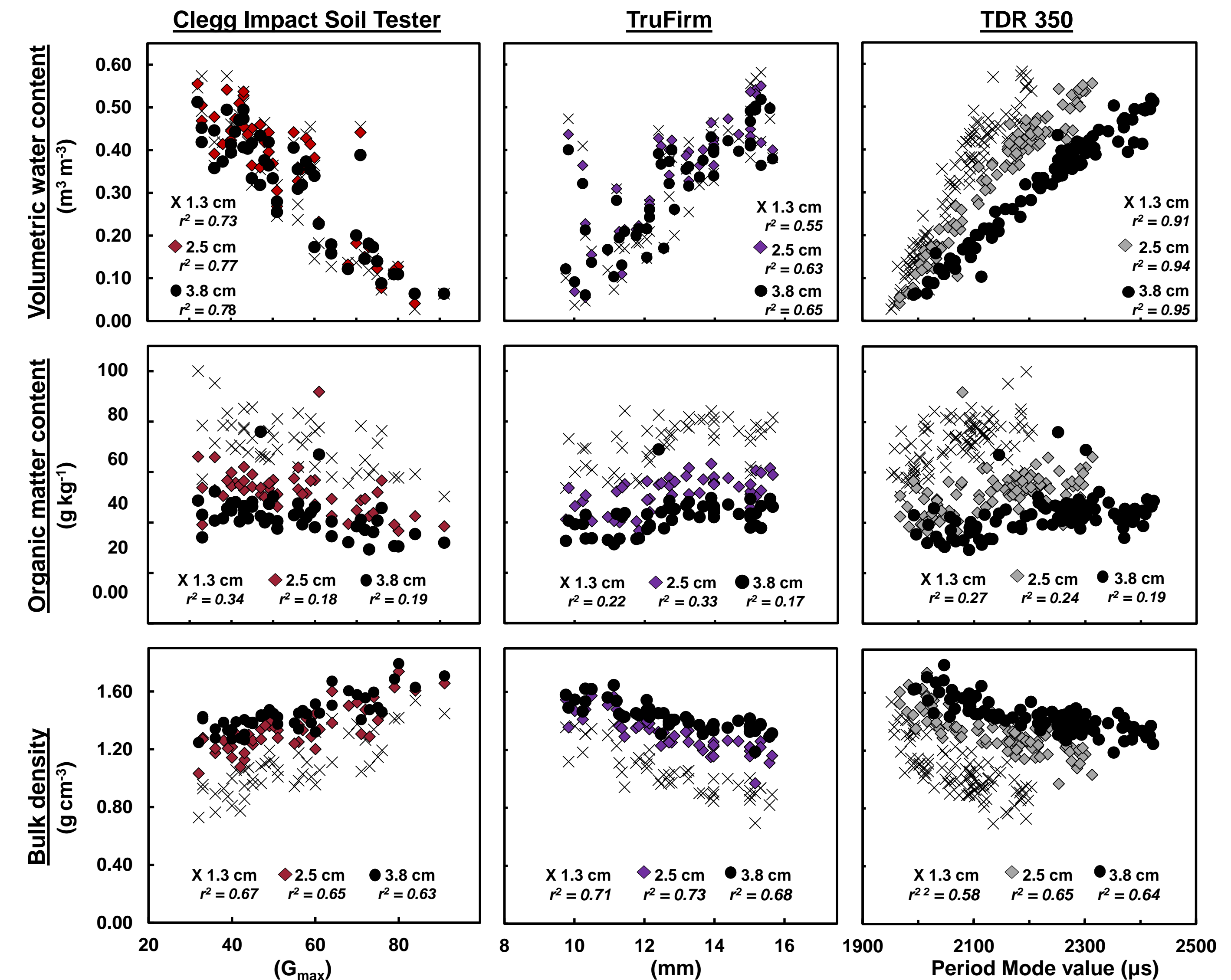
Fig. 2: The relationships between measurement devices and ground truth data for volumetric water content, organic matter content, and bulk density within the uppermost 1.3, 2.5, and 3.8 cm of a creeping bentgrass, USGA sand-based putting green.
